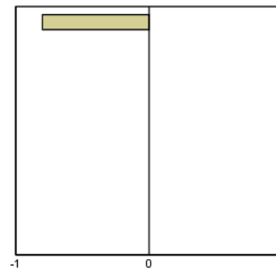
ARIMA(1,0,0), \phi < 0
