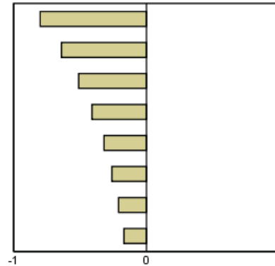
ARIMA(1,0,0), \phi > 0
