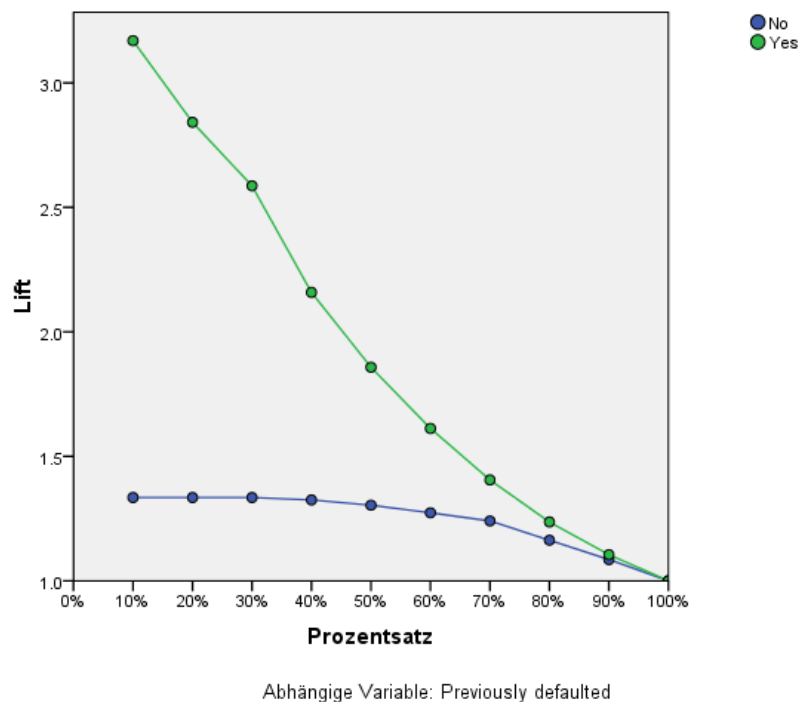
Abbildung 4-20 Lift Chart (Index)
