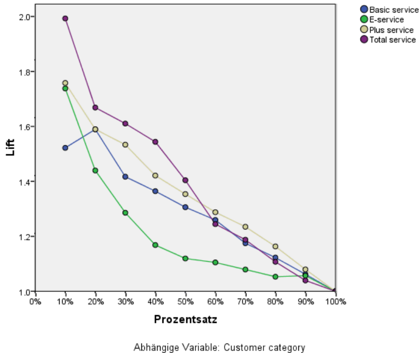
Abbildung 5-14 Lift Chart (Index)
