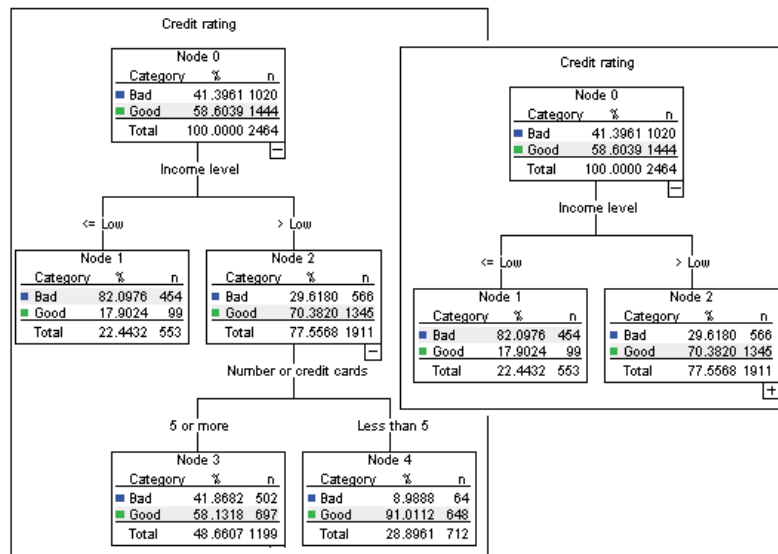
Figure 2-1 Expanded and collapsed tree
